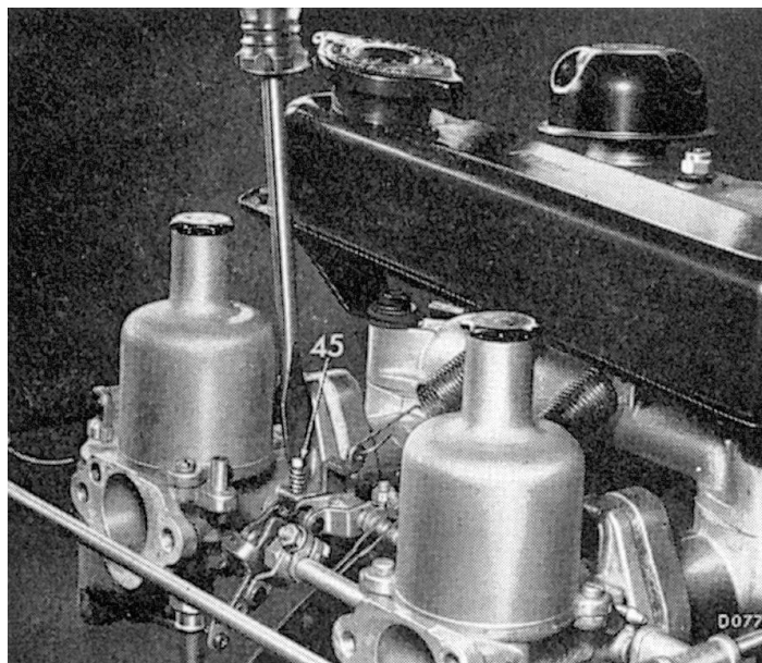
Fig. 20. Adjusting throttle stop screws
